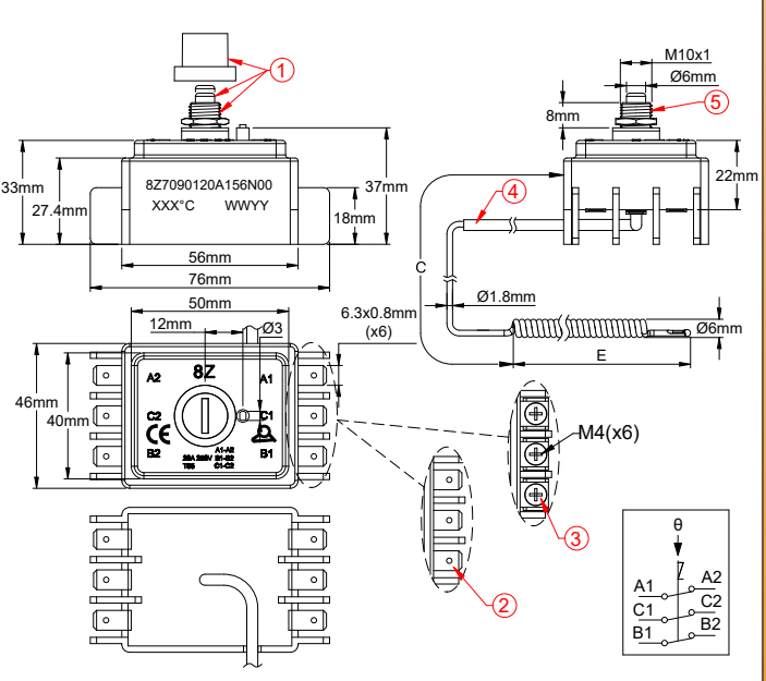
Mounting by M10x1 front bushing, horizontal terminals, type 8Z1 and 8Z7
